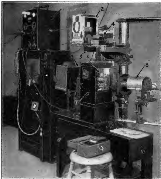
FIG. 2. Complete microcinematographic apparatus. (1) Camera timer with motor, (2) camera, (3) observation piece, (4) focusing device, (5) microscope, (6) incubator, (7) incandescent lamp, (8) arc lamp, (9) electric exposure meter.
